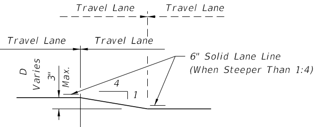
TRAVEL LANE TREATMENT FOR MILLING OR RESURFACING DETAIL (1:4 Slope Shown, See Note 5)
