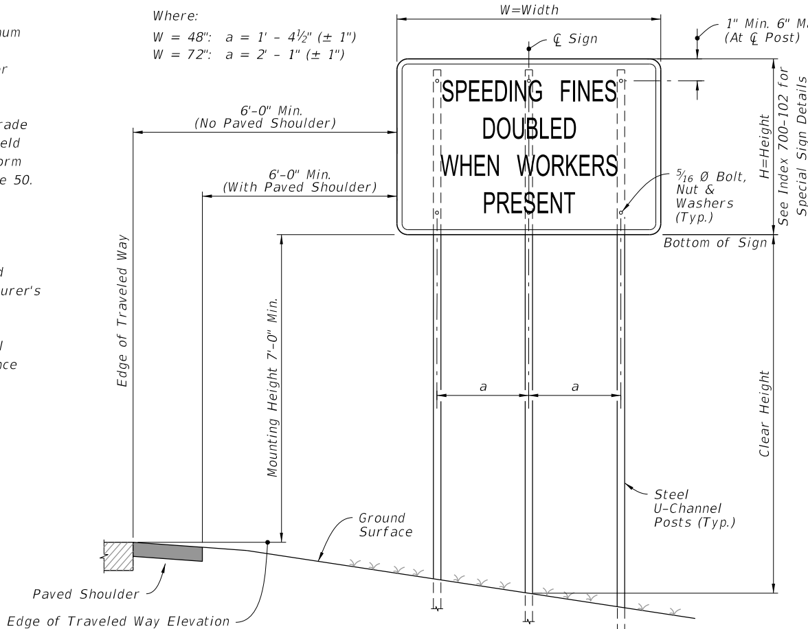
3 POST SIGN SUPPORT MOUNTING DETAILS
