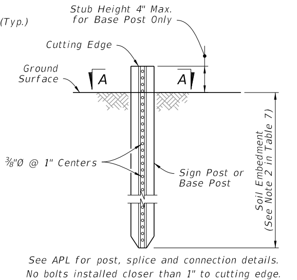
FOUNDATION DETAIL
