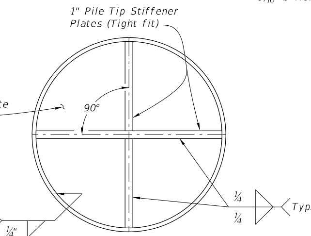
VIEW C-C PILE TIP DETAIL
