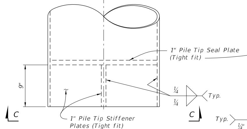
VIEW B-B
