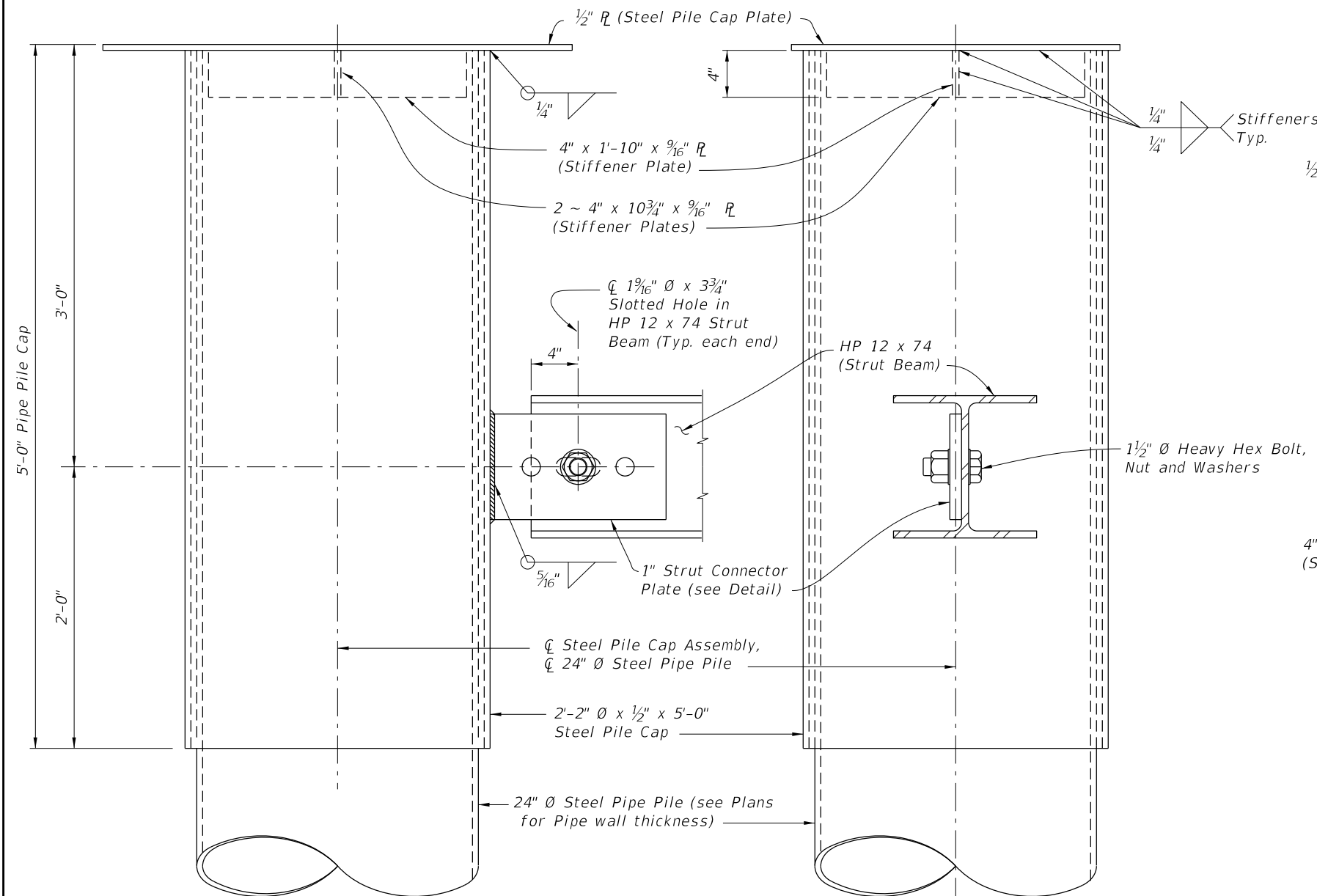
PARTIAL VIEW A-A
