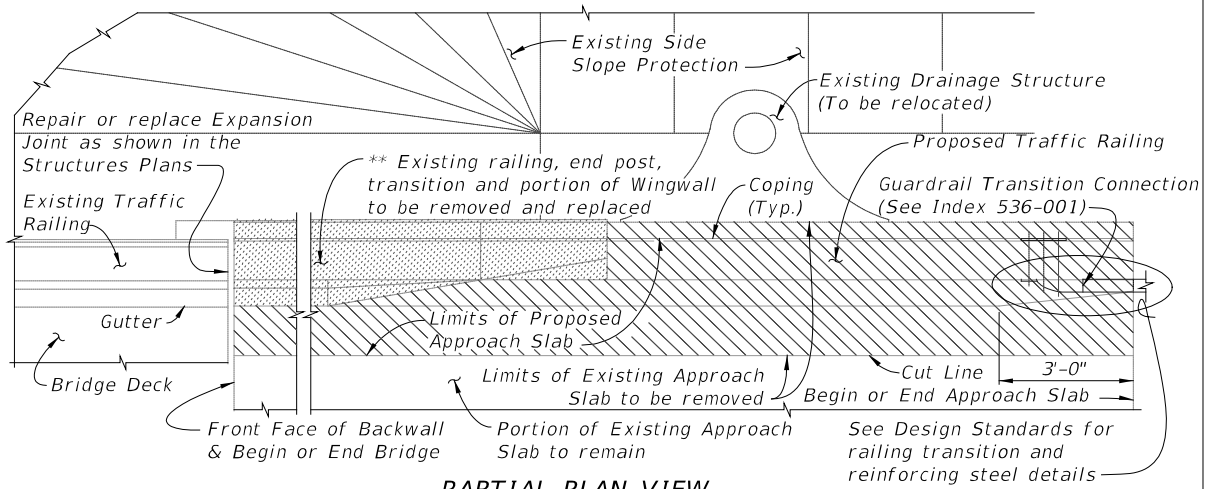
PARTIAL PLAN VIEW (Existing W-Beam Guardrail to be removed not shown for clarity. "F" Shape Railing shown, "New Jersey" Shape Railing similar.)
