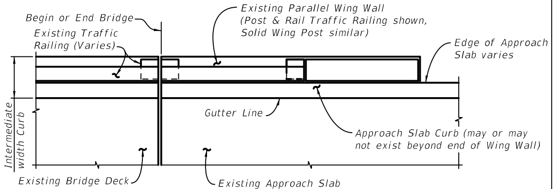
PARTIAL PLAN VIEW OF EXISTING BRIDGE WITH INTERMEDIATE WIDTH CURBS AND PERPENDICULAR OR ANGLED WING WALLS - USE INDEX 460-474, SCHEME 2
