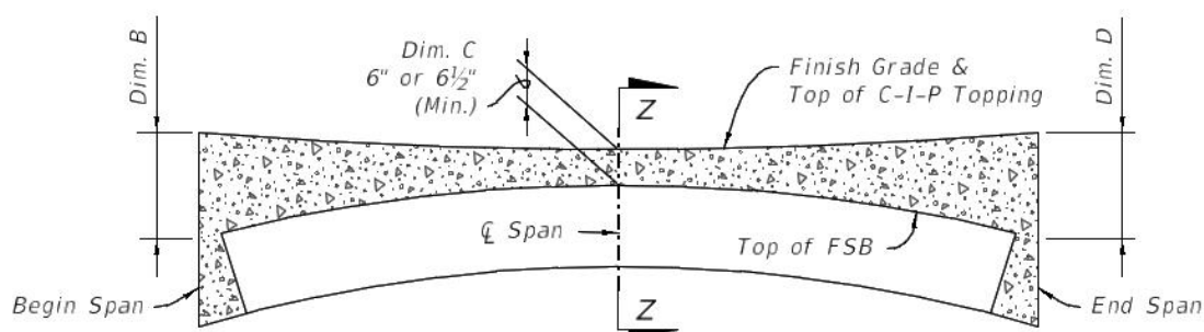
TOPPING DIAGRAM FOR SAG VERTICAL CURVE SPANS CONTROL AT \bar{C} SPAN (CASE 2)
