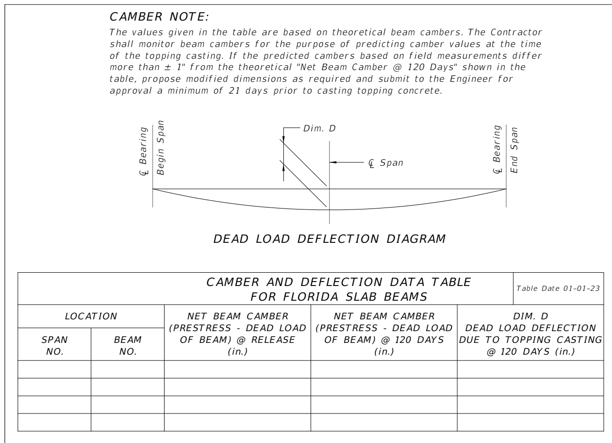
Figure 11 Dead Load Deflection Data Table, Diagram and Note
