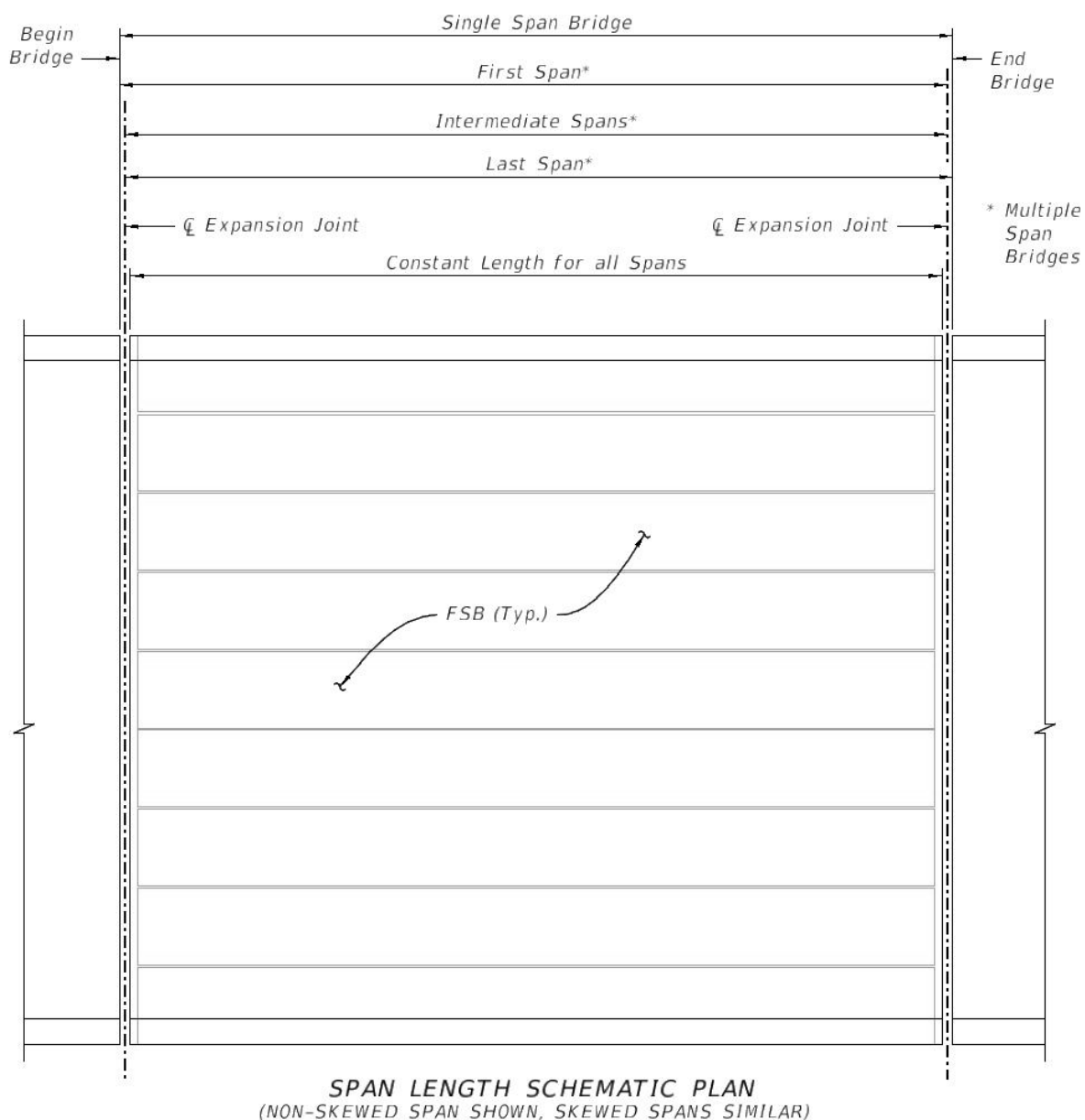
Figure 1 Span Length Schematic Plan
