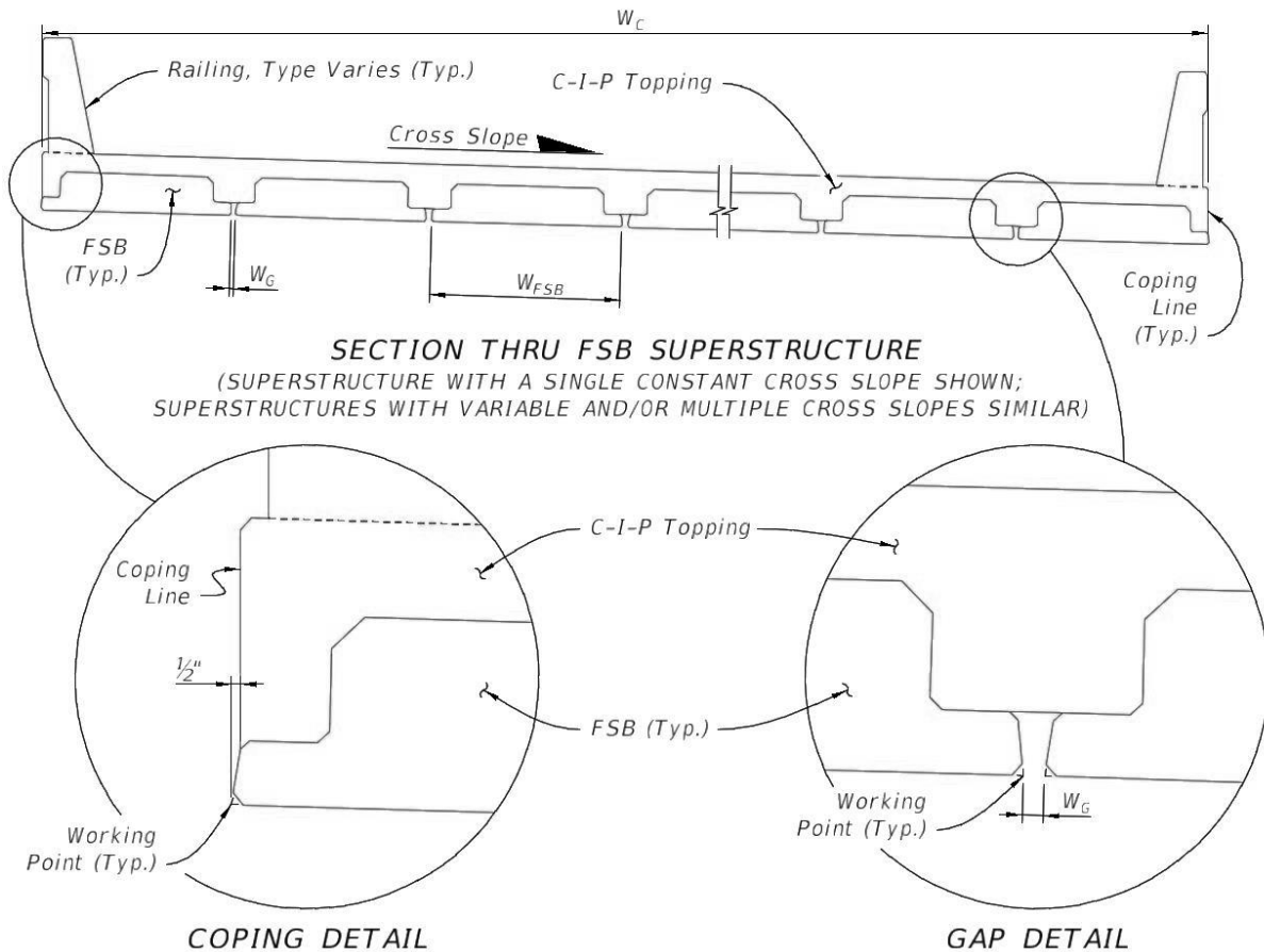
Figure 3 Section Through FSB Superstructure
