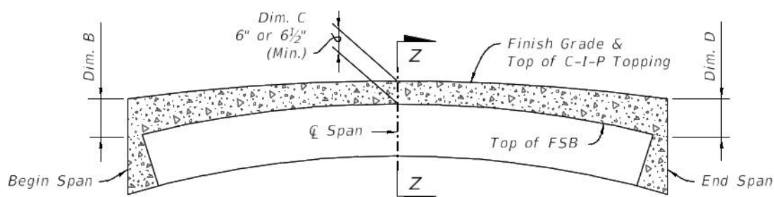
TOPPING DIAGRAM FOR CREST VERTICAL CURVE SPANS CONTROL AT \bar{C} SPAN (CASE 3)
