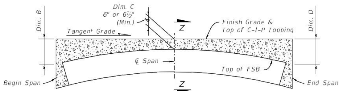
TOPPING DIAGRAM FOR TANGENT SPANS CONTROL AT \bar{C} SPAN (CASE 1)
