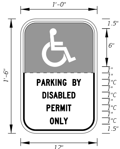
FTP-017-25 1'-0" X 1'-6" 1.5" Radii 3/8" Border TOP: Blue Background White Border BOTTOM: 1" Series C Legend White Background Black Legend and Border
