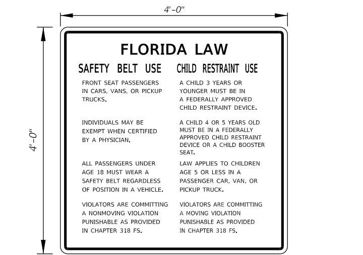
FTP-006-25 4'-0" X 4'-0" 1.5" Radii 0.4" Border 2.5" Series C Legend 2" Series C Legend 1.5" Series C Legend and White Background Black Legend and Border
