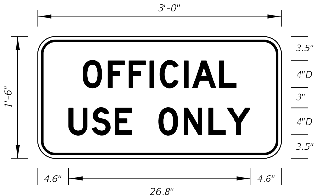
FTP-013-25 3'-0" X 1'-6" 1.5" Radii 3/4" Border 4" Series D Legend White Background Black Legend and Border
