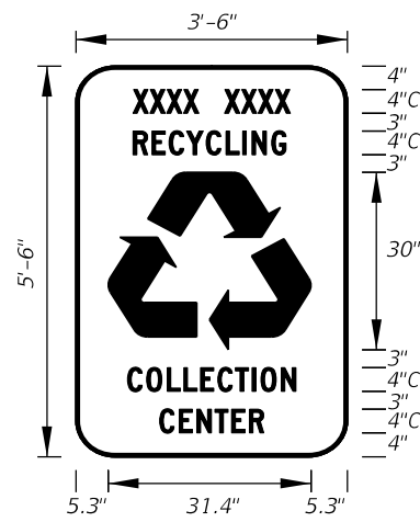
FTP-608-25 3'-6" X 5'-6" 3" Radii 2" Border 4" Series C Legend Green Background Municipality Name Optional White Legend, Border and Symbol
