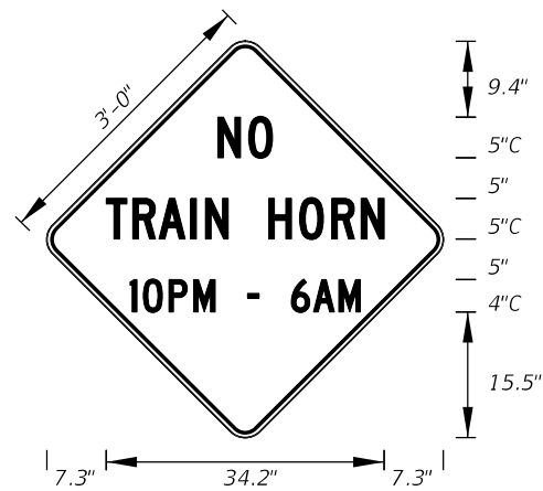
FTP-203A-25 3'-0" X 3'-0" 1.5" Radii 3/4" Border 4" and 5" Series C Legend Yellow Background Black Legend and Border
