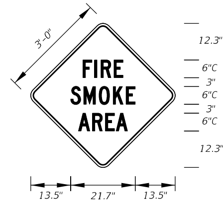
FTP-208-25 3'-0" X 3'-0" 1.5" Radii \frac{3}{4} " Border
