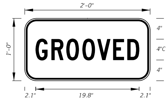
FTP-014-25 2'-0" X 1'-0" 1.5" Radii 5/8" Border 4" Series C Legend Yellow Background Black Legend and Border
