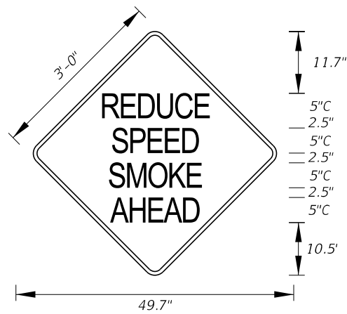
TTC-019-25 3'-0" x 3'-0" 1.5" Radii 3/4" Border 5" Series C Legend Pink Background Black Legend and Border
