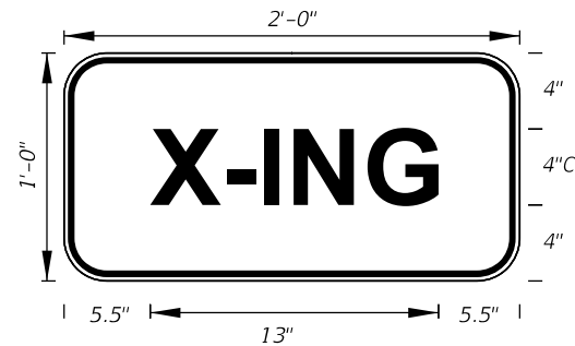
FTP-204-25 2'-0" X 1'-0" 1.5" Radii 3/4" Border 4" Series C Legend Yellow Background Black Legend and Border
