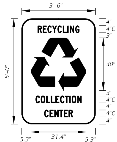
FTP-607-25 3'-6" X 5'-0" 1.5" Radii 2" Border 4" Series C Legend Green Background White Legend, Border and Symbol
