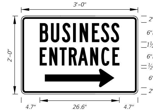
TTC-016R-25 TTC-016L-25 3'-0" X 2'-0" 1.5" Radii 3/4" Border 6" Series B Legend Blue Background White Legend and Border NOTE: Use TTC-016L-25 for "LEFT ARROW".
