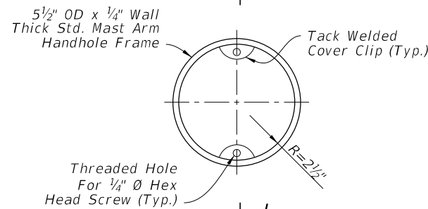
HANDHOLE FRAME
