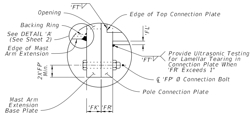
DETAIL 'C'
