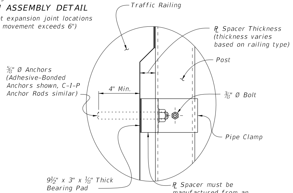
DETAIL "A"
