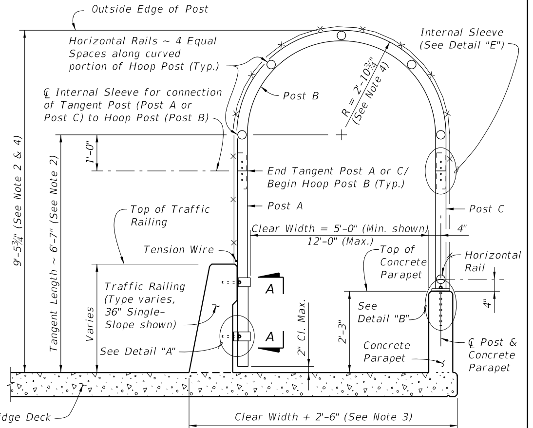
TYPICAL SECTION
