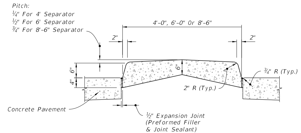
TRANSVERSE SECTION
