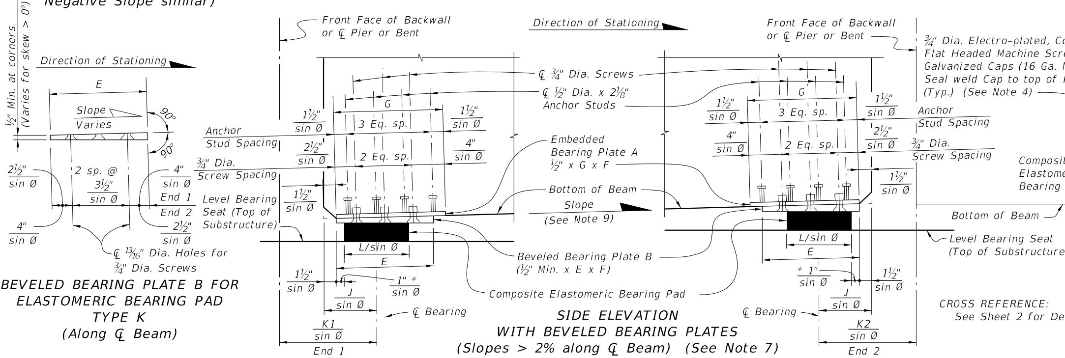
BEVELED BEARING PLATE B FOR ELASTOMERIC BEARING PAD TYPE K (Along \bar{C} Beam) (Slopes > 2% along \bar{C} Beam) (See Note 7)
