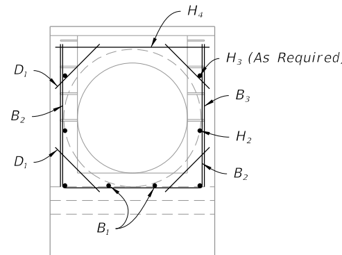
END VIEW
