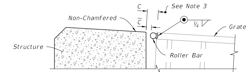
DETAIL "A"
