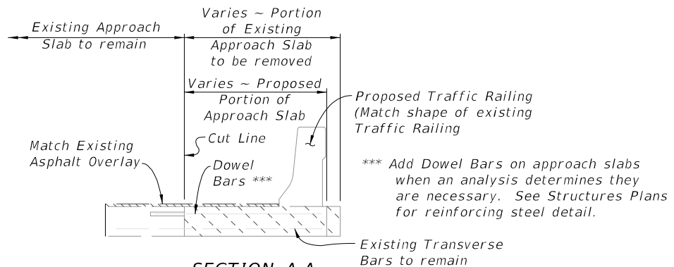
SECTION A-A (Showing one layer of existing reinforcement)
