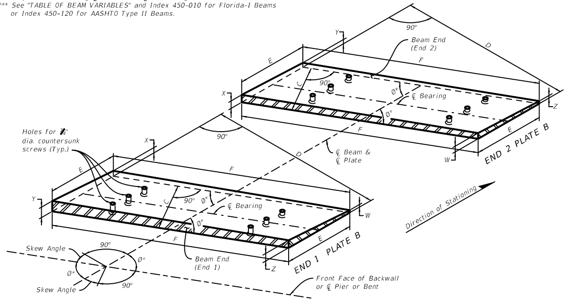
ISOMETRIC VIEW OF BEVELED BEARING PLATES (TYPE 1) FOR FLORIDA I-BEAMS (SKEWED PLATES SHOWN, NON-SKEWED PLATES AND AASHTO TYPE II BEAMS SIMILAR)
