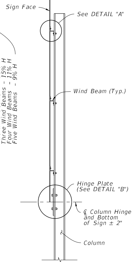
SIDE ELEVATION
