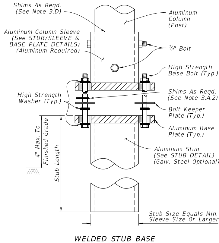
WELDED STUB BASE
