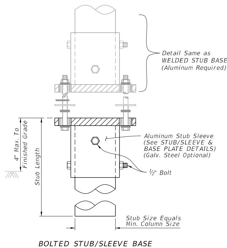
BOLTED STUB/SLEEVE BASE
