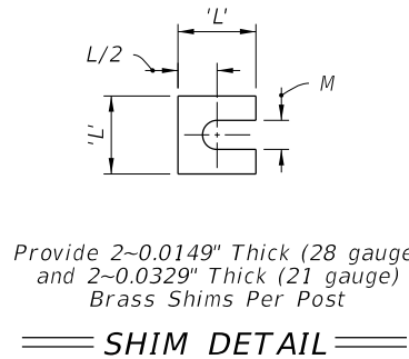
SHIM DETAIL
