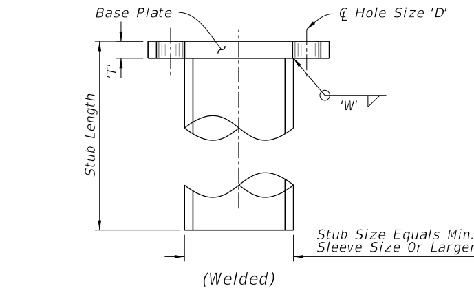
STUB DETAIL
