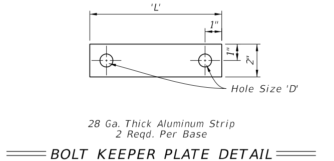
BOLT KEEPER PLATE DETAIL
