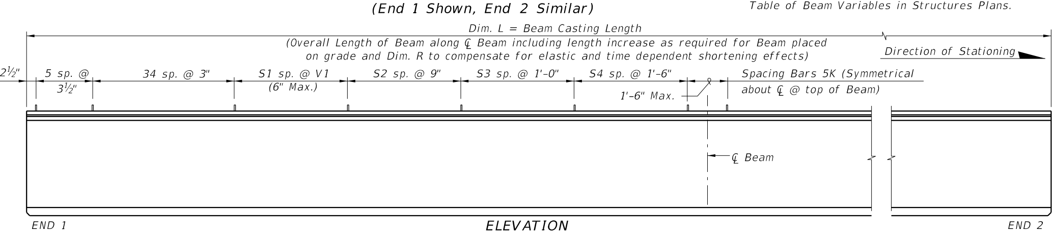
ELEVATION AT END OF BEAM (Flanges Not Shown For Clarity) (End 1 Shown, End 2 Similar)
