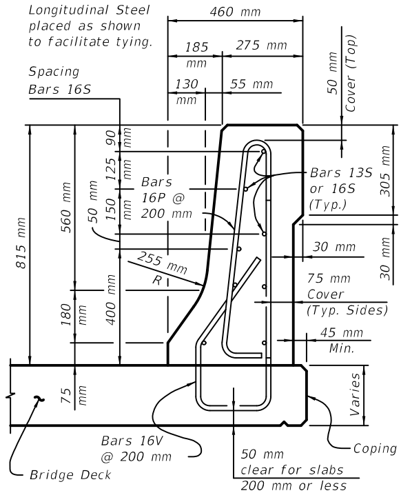
TYPICAL SECTION THRU F SHAPE RAILING (Metric with soft converted rebar) INDEX NO. 700
