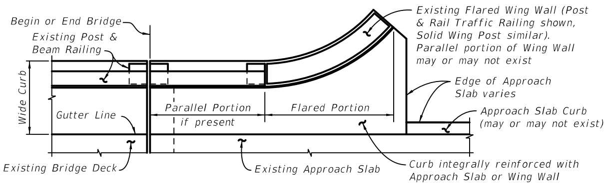
PARTIAL PLAN VIEW OF EXISTING BRIDGE WITH WIDE CURBS, FLARED WING WALLS AND PARALLEL INTEGRALLY REINFORCED APPROACH SLAB CURBS - USE SCHEME 2
