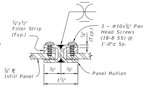
SECTION C-C PANEL/SPLICE CONNECTION
