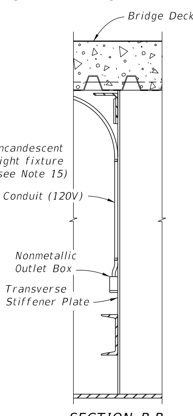
LIGHTING DETAILS FOR STEEL BOX GIRDER BRIDGE
