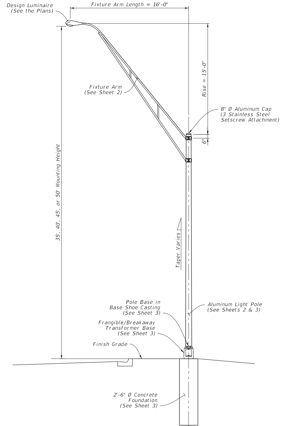
LIGHT POLE - ELEVATION
