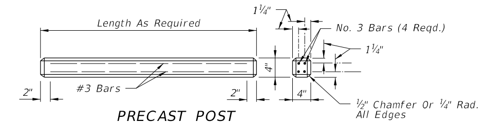
PRECAST POST
