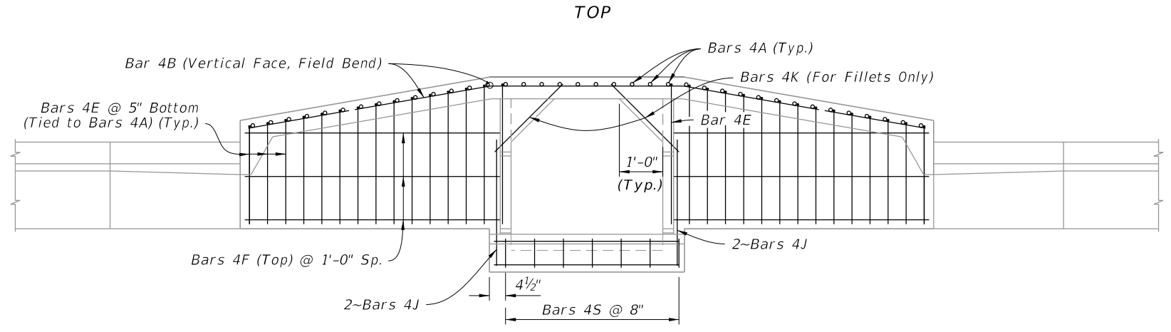
TYPE 6 REINFORCING DETAILS
