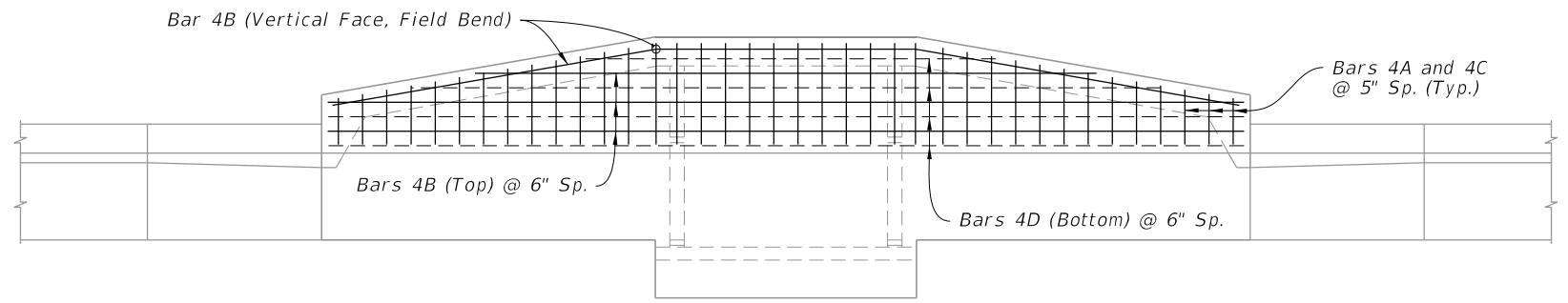
TYPE 5 REINFORCING DETAILS
