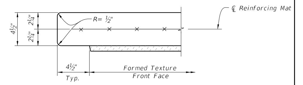
DETAIL "B" - TOP-INSTALLED (Typ. Both Ends)
