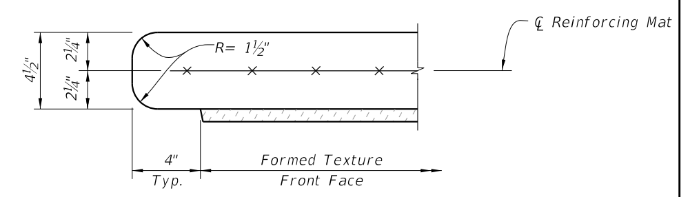
DETAIL "B" - SIDE-INSTALLED (Typ. Both Ends)
