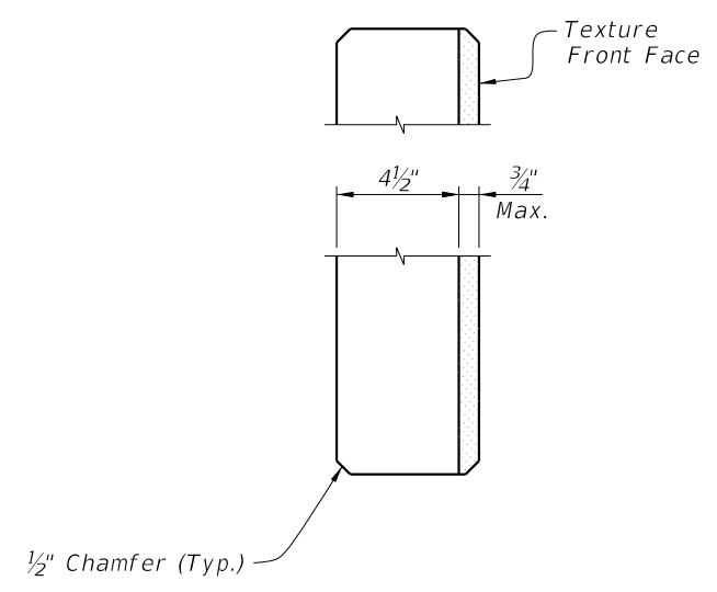
SECTION F-F
