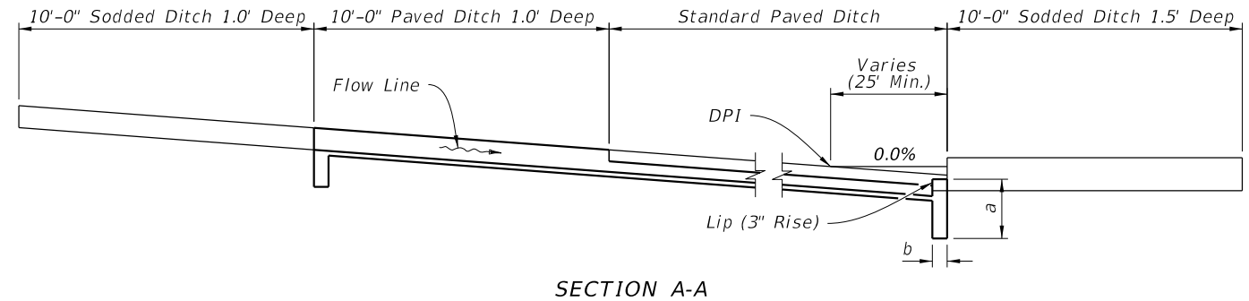
PAVED DITCH END TREATMENT
