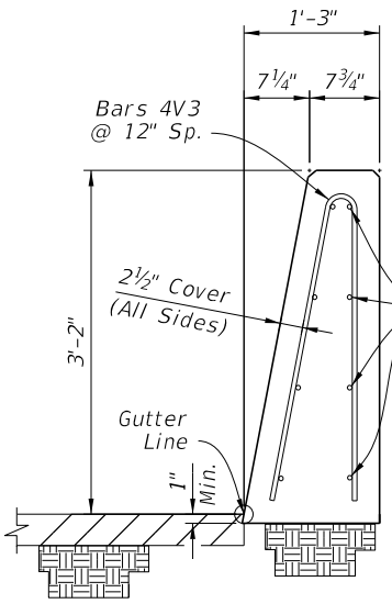
SECTION A-A 38" HEIGHT SINGLE-FACED SECTION (Reverse Side Similar by Opposite Hand)
