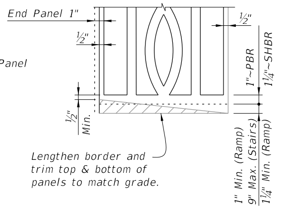
PANEL ADJUSTMENT FOR RAILINGS ON GRADES
