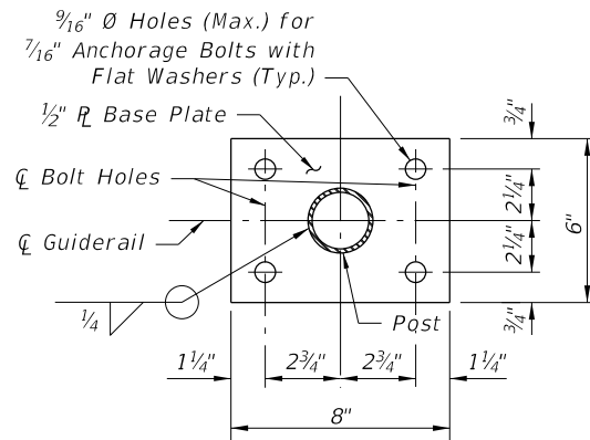
SECTION C-C BASE PLATE DETAIL (4~Bolt Anchorage)
