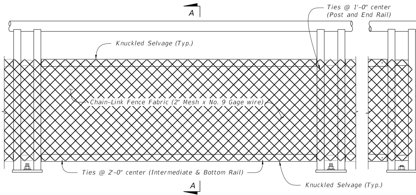
TYPE 2 - CHAIN-LINK (Continuous Infill Panel)
