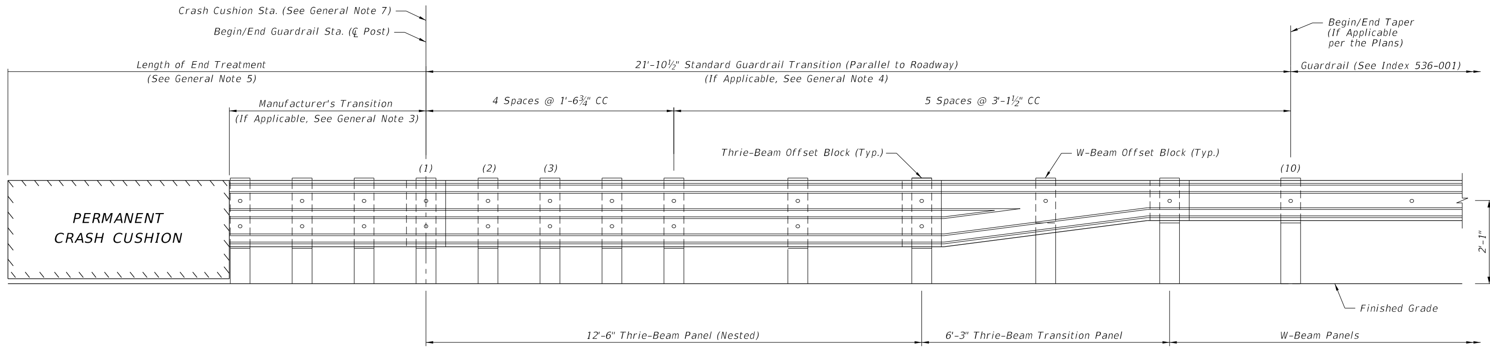
ELEVATION VIEW
