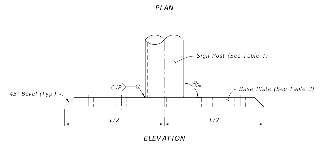
SIGN SUPPORT WELDMENT DETAIL (Staggered Anchor Rod Pattern shown)
