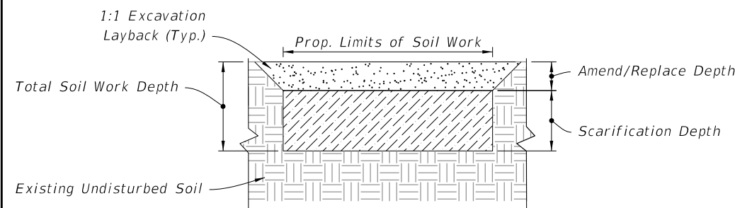
(Typical Section)
