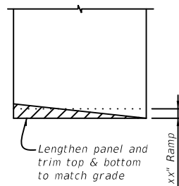
PANEL ADJUSTMENT FOR RAILINGS ON GRADES STEEPER THAN 5%
