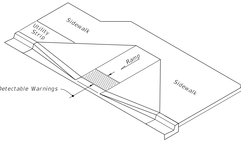
ISOMETRIC VIEW
