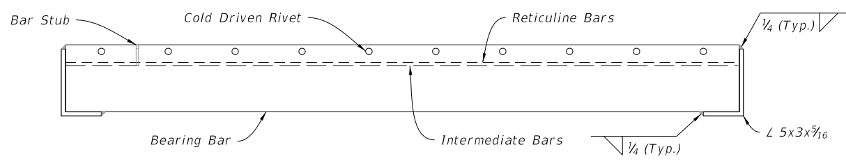
SECTION C-C
