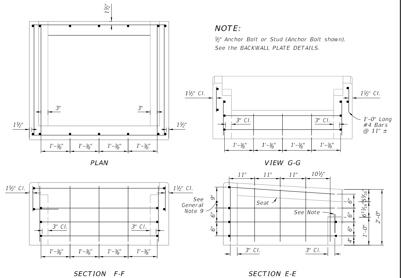
REINFORCING DETAILS
