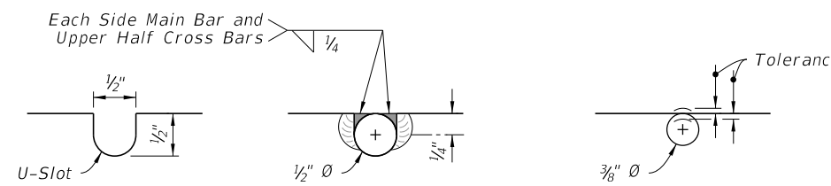
WELDED
