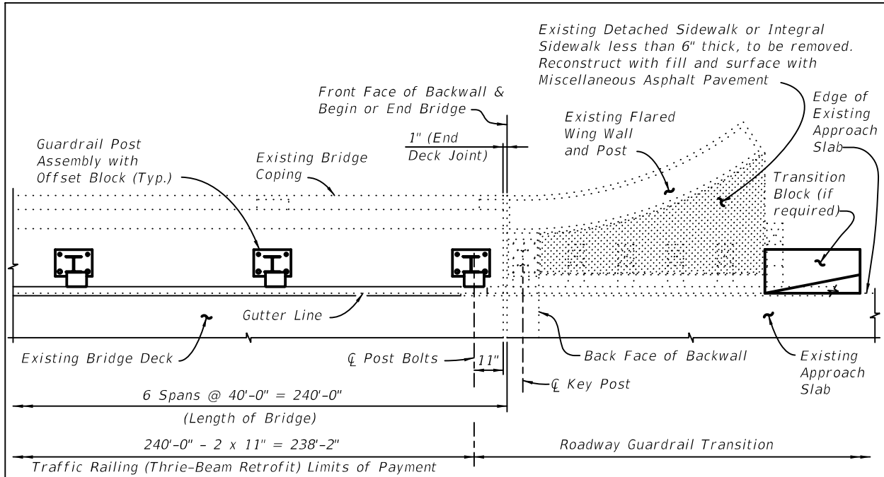
EXAMPLE QUANTITY CALCULATION - CASE II ▶ Direction of Traffic (INDEX 460-472 SCHEME 2 SHOWN, INDEX 460-471, 460-472, 460-473, 460-474, 460-475 AND 460-476 SCHEME 1 AND INDEX 460-473 AND 460-476 SCHEME 2 SIMILAR)
