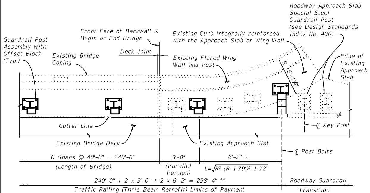
EXAMPLE QUANTITY CALCULATION - CASE III ▶ Direction of Traffic (INDEX 460-472 SCHEMES 3 AND 4 SHOWN, INDEX 460-473, 460-475 AND 460-476 SCHEMES 3 AND 4 AND INDEX 460-474 SCHEME 3 SIMILAR)
