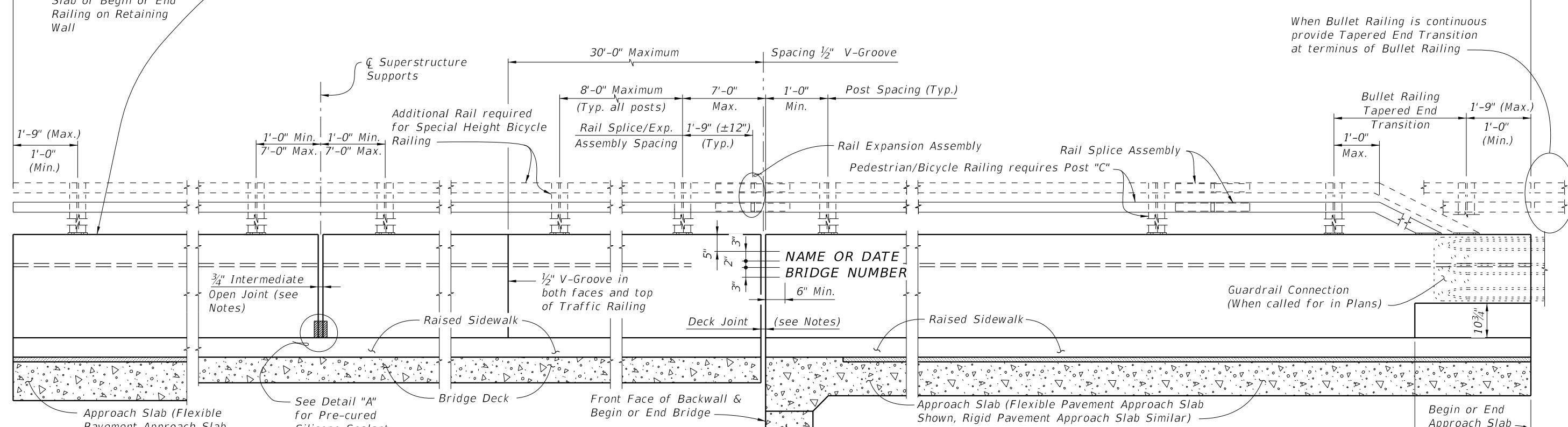
ELEVATION OF INSIDE FACE OF RAILING (Reinforcing Steel not shown for clarity) TRAFFIC RAILING NOTES
