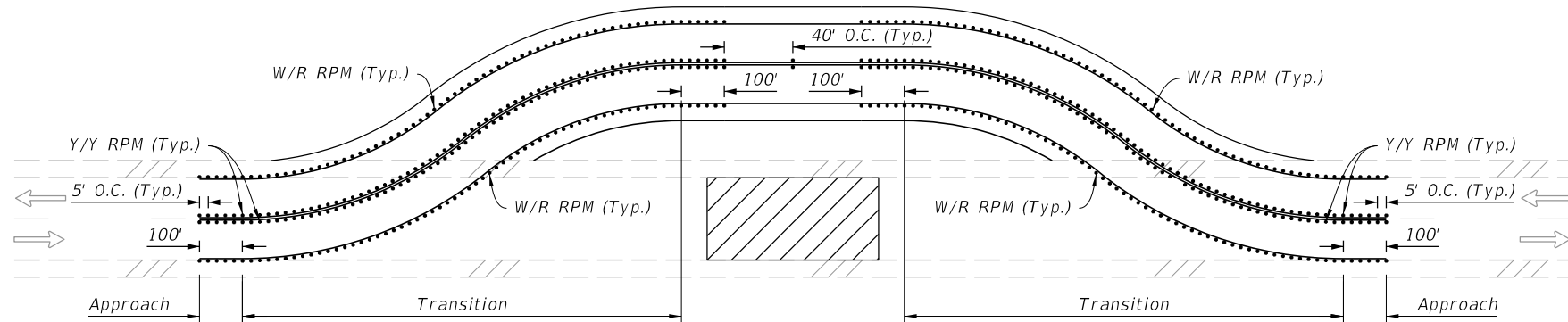
RPM PLACEMENT ON TWO-LANE ROADWAYS
