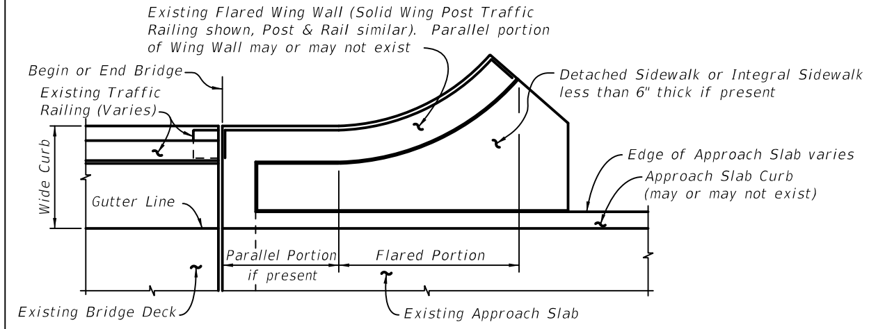
PARTIAL PLAN VIEW OF EXISTING BRIDGE WITH WIDE CURBS, FLARED WING WALLS AND APPROACH SLABS WITH DETACHED SIDEWALKS OR SIDEWALKS LESS THAN 6" THICK - USE INDEX 521-482, SCHEME 5
