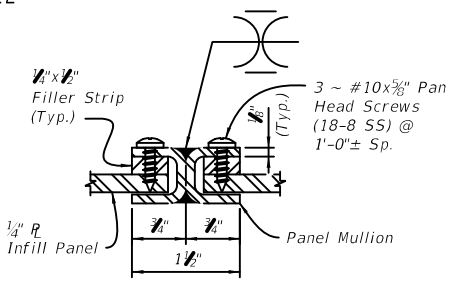
SECTION C-C PANEL/SPLICE CONNECTION
