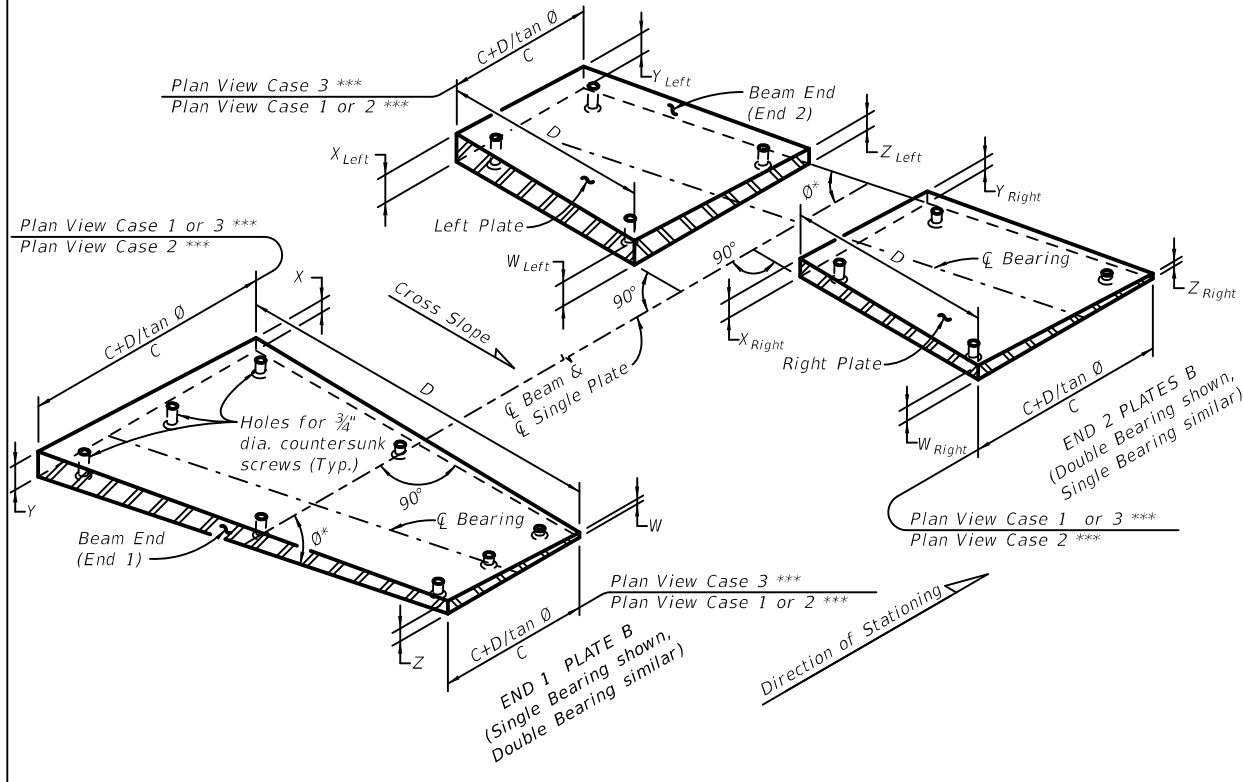
ISOMETRIC VIEW OF BEVELED BEARING PLATES FOR FLORIDA-U BEAMS (SKEWED PLATES SHOWN, NON-SKEWED PLATES SIMILAR)
