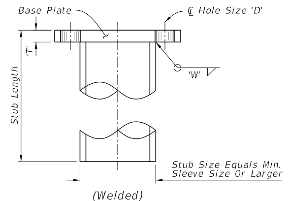
STUB DETAIL
