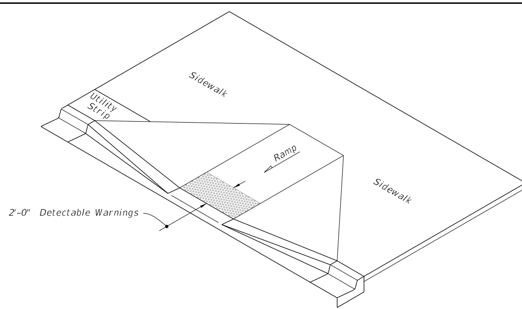
ISOMETRIC VIEW
