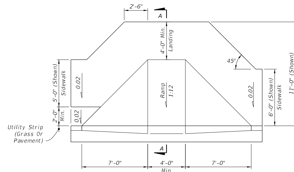
PLAN VIEW
