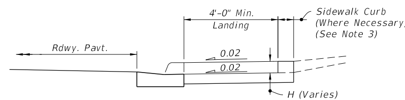
SECTION E-E
