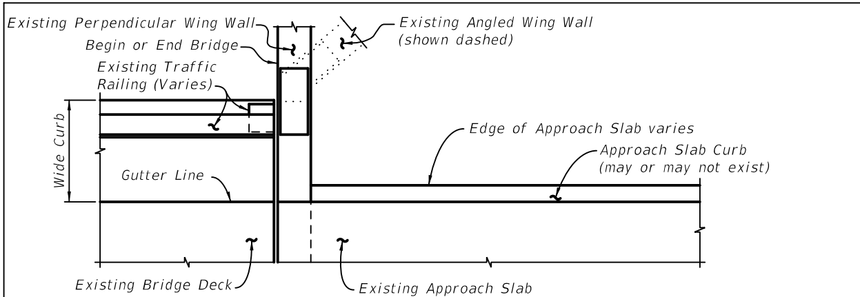
PARTIAL PLAN VIEW OF EXISTING BRIDGE WITH WIDE CURBS AND PERPENDICULAR OR ANGLED WING WALLS - USE INDEX 521-482, SCHEME 1
