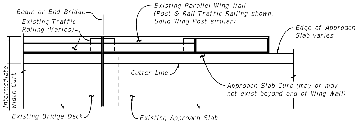
PARTIAL PLAN VIEW OF EXISTING BRIDGE WITH INTERMEDIATE WIDTH CURBS, PARALLEL WING WALLS AND PARALLEL INTEGRAL APPROACH SLAB CURBS - USE INDEX 521-483, SCHEME 2
