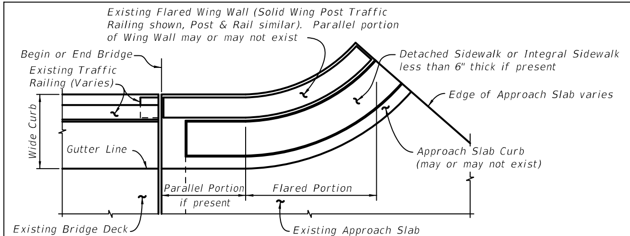
PARTIAL PLAN VIEW OF EXISTING BRIDGE WITH WIDE CURBS, FLARED WING WALLS AND APPROACH SLABS WITH DETACHED SIDEWALKS OR SIDEWALKS LESS THAN 6" THICK - USE INDEX 521-482, SCHEME 4
