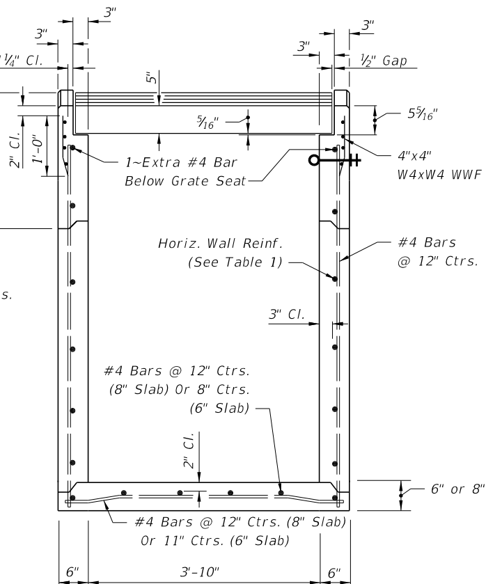
(Pipe Opening Not Shown) SECTION AA (PRECAST INLET)
