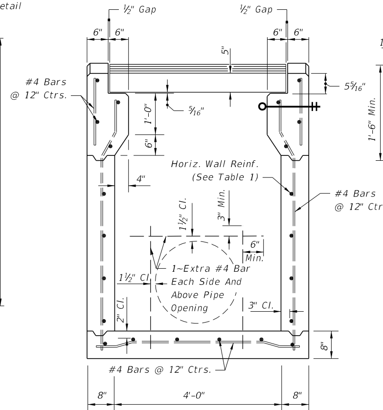
(Pipe Opening Shown) SECTION AA (CAST-IN-PLACE INLET)
