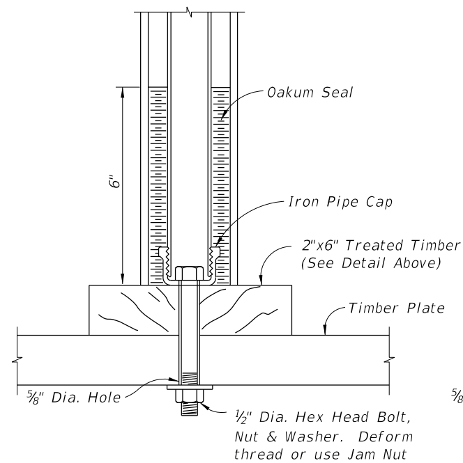
TIMBER PLATE
