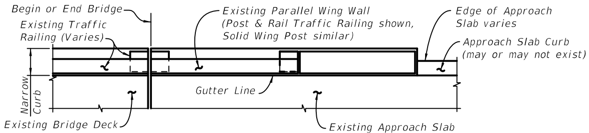
PARTIAL PLAN VIEW OF EXISTING BRIDGE WITH NARROW CURBS AND PARALLEL WING WALLS - USE INDEX 460-471, SCHEME 2
