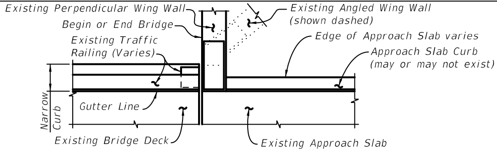
PARTIAL PLAN VIEW OF EXISTING BRIDGE WITH NARROW CURBS AND PERPENDICULAR OR ANGLED WING WALLS - USE INDEX 460-471, SCHEME 1
