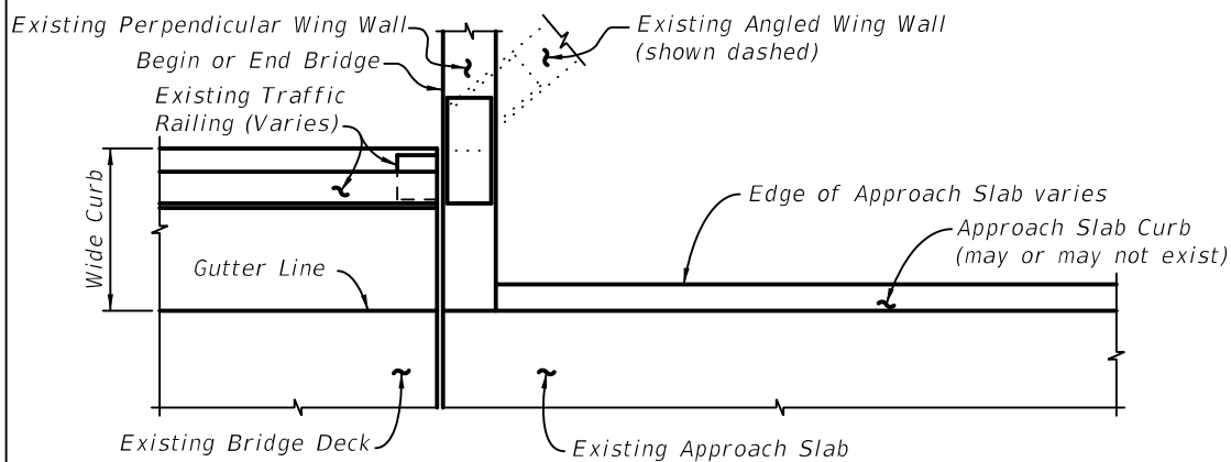
PARTIAL PLAN VIEW OF EXISTING BRIDGE WITH WIDE CURBS AND PERPENDICULAR OR ANGLED WING WALLS - USE INDEX 460-472, 460-473, 460-475 OR 460-476, SCHEME 1
