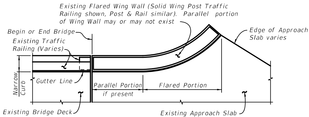
PARTIAL PLAN VIEW OF EXISTING BRIDGE WITH NARROW CURBS AND FLARED WING WALLS - USE INDEX 460-471, SCHEME 3
