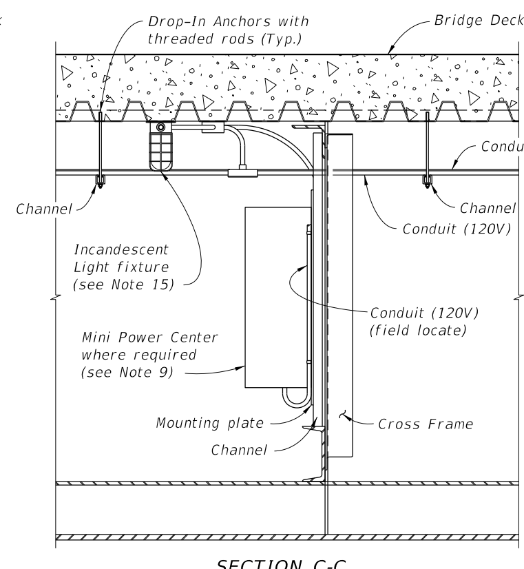
SECTION C-C
