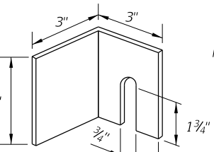
ANGLE DETAIL
