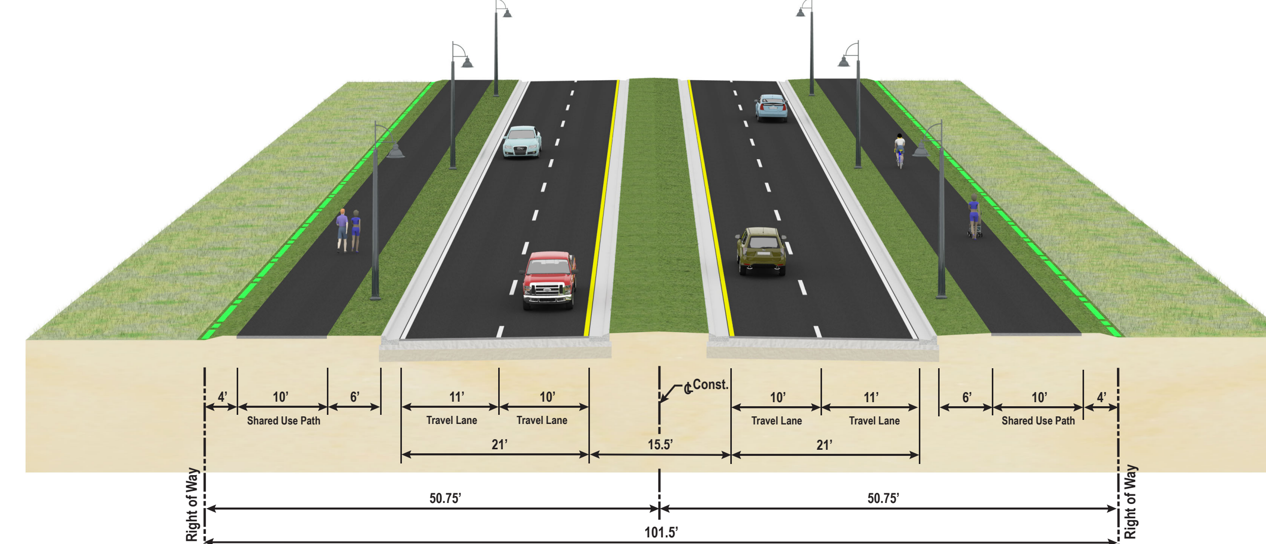
Typical Section - Segment 2 Alternative 2C from Avalon Drive to SR 5/US 1 (Federal Hwy.)
