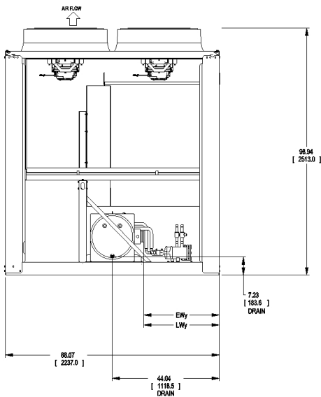
NON-CONTROL PANEL END VIEW
