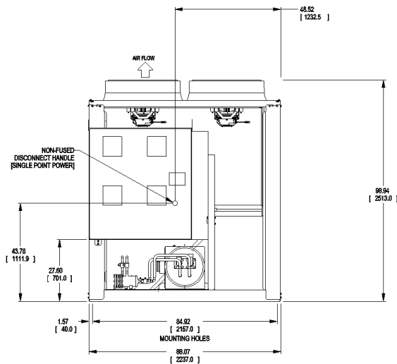
CONTROL PANEL END VIEW
