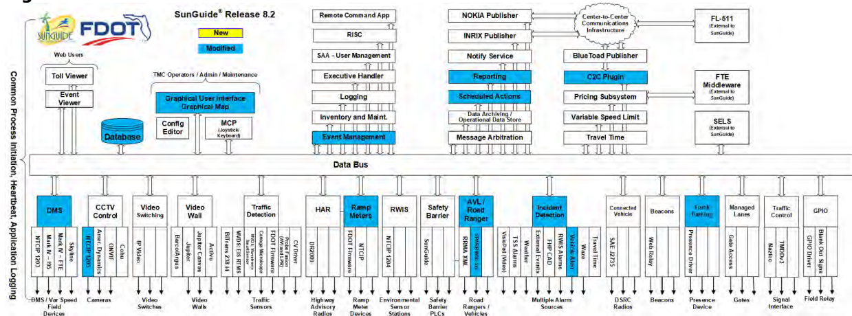
Figure 1: SunGuide Software Architecture
