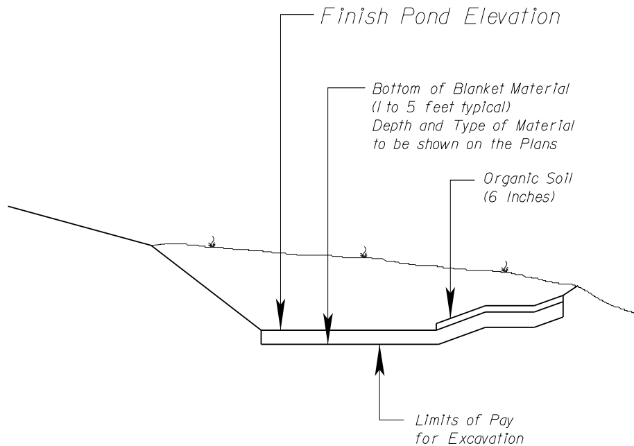
Figure 3.5.1 Pond Template
