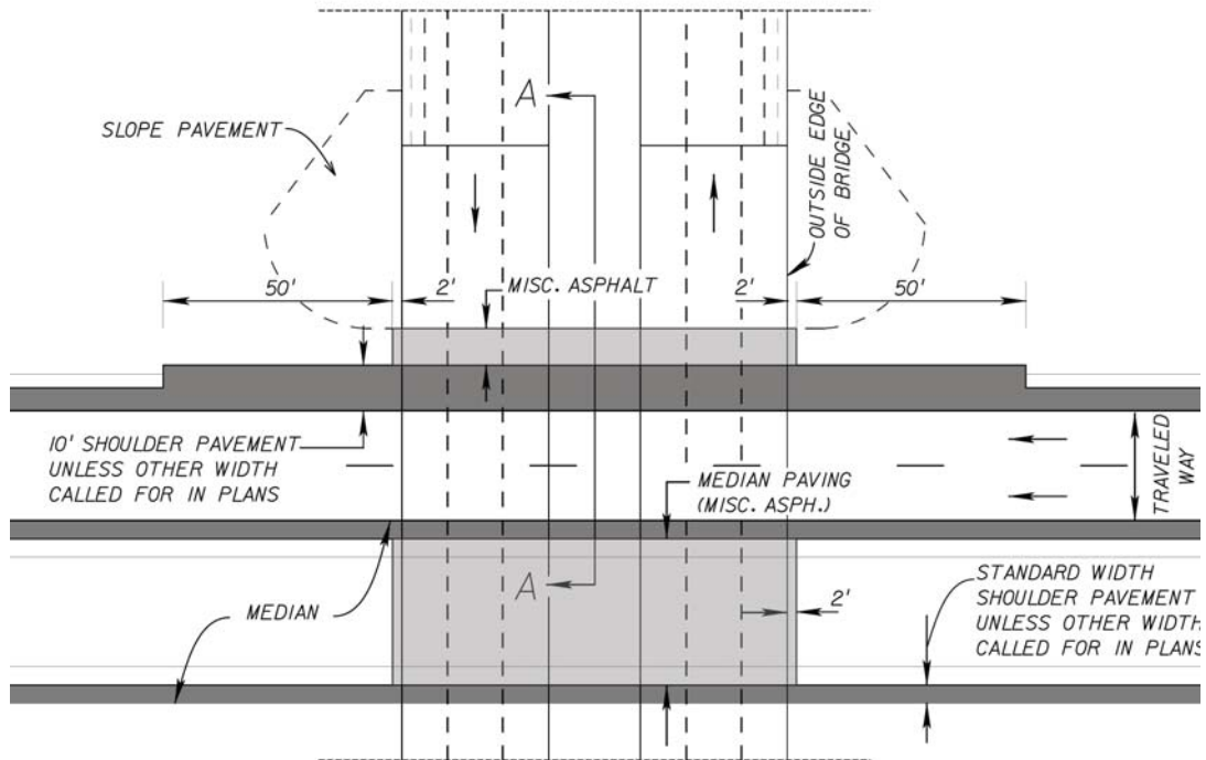
Figure 2.3.2 Typical Paving Under Bridge
